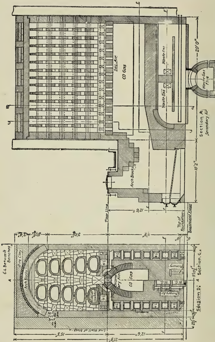
From "Coal and Coke," by F. H. Wagner. Fig. 86.—Horizontal Gas-Works Retort.
